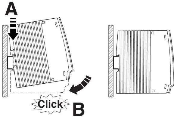
Figure 7 Assembly on standard DIN rail
